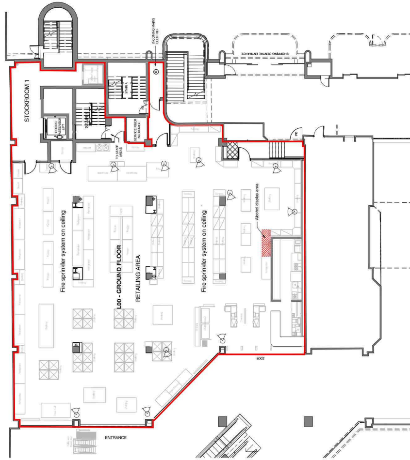
1 Proposed Ground Floor Plan
